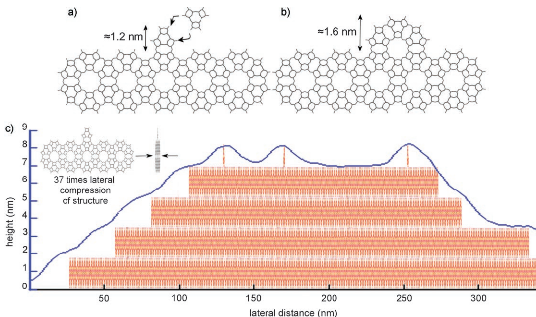
Figure 3. a) An individual cancrinite column sits 1.20 nm proud of the (100) side wall. b) Connected cancrinite columns sit 1.6 nm proud of the (100) side wall. c) Illustration of the 37-fold lateral compression in effect observed by AFM owing to the superior vertical resolution. Superimposed, the blue line shows the AFM cross-section, from Figure 2b, which is a measure of the surface structure convoluted with the tip profile.
